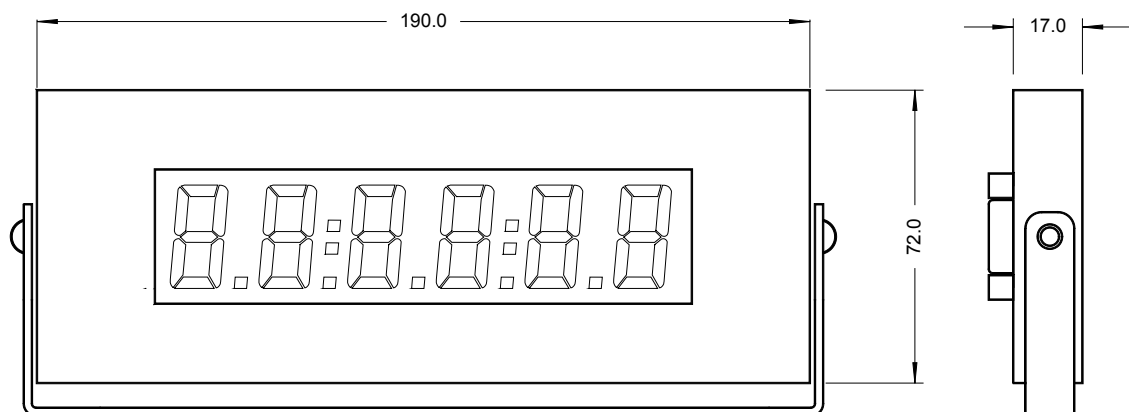
DIMENSIONS (in metric millimetres, 6 digit version shown)
